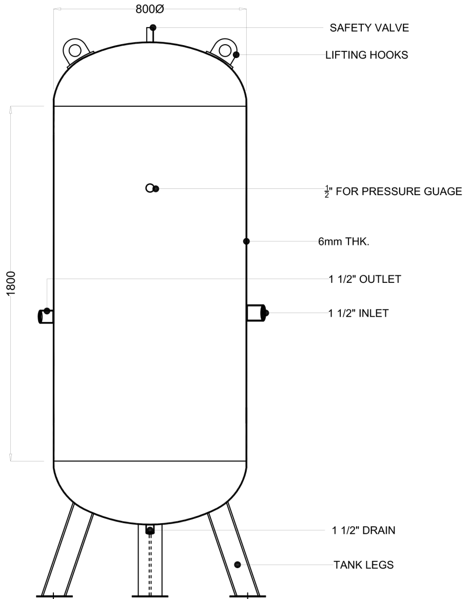
1 1000Ltr AIR RECEIVER TANK
