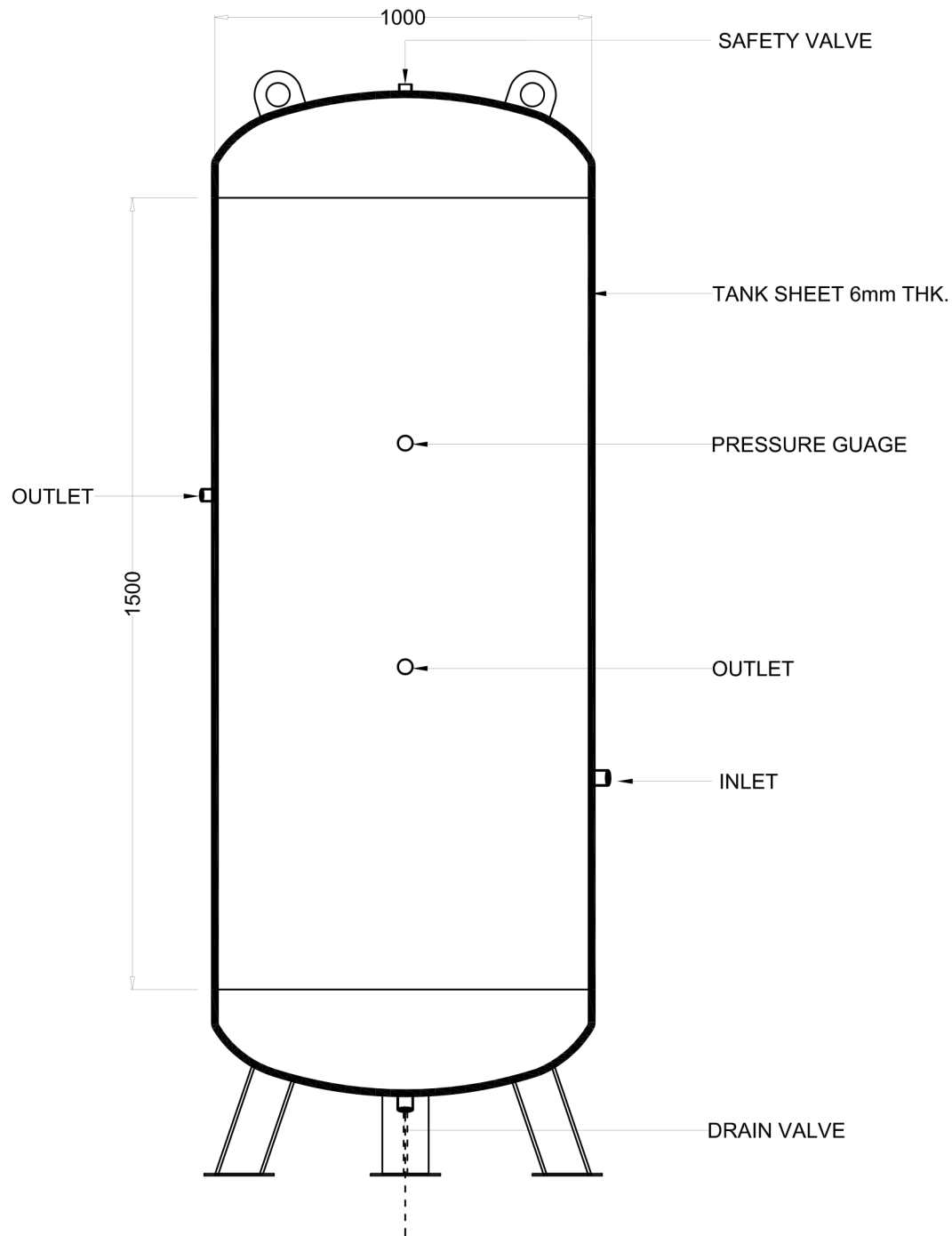
1500ltr AIR RECEIVER TANK
