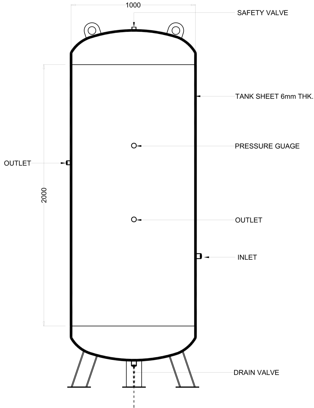
2000ltr AIR RECEIVER TANK
