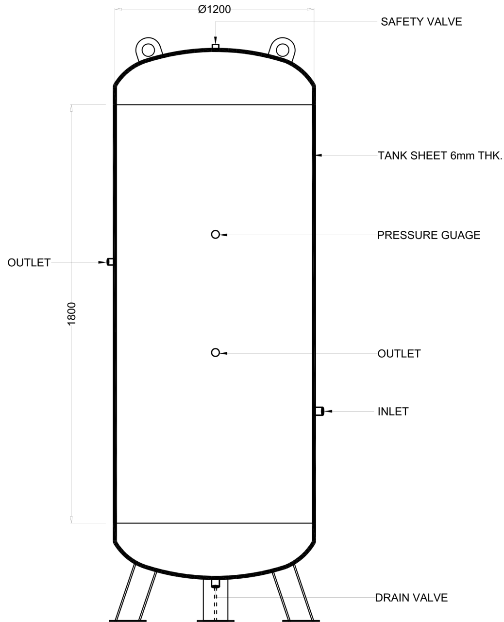
2500ltr AIR RECEIVER TANK
